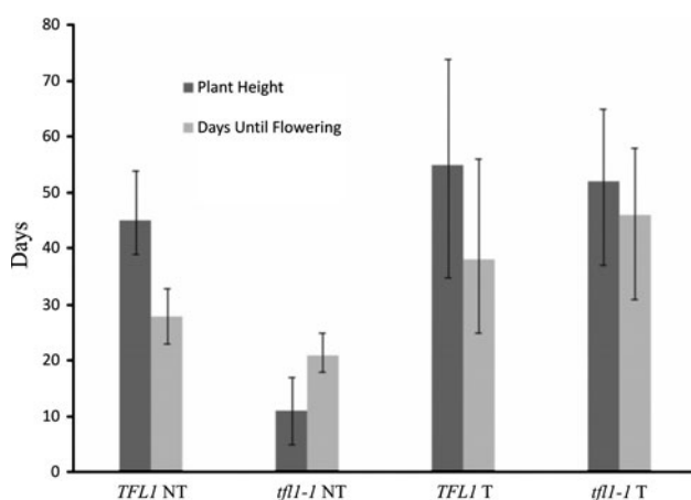
Fig. 4 Average number of days until flowering and average plant height observations for transformed ( T ) and nontransformed ( NT ), TFLI (indeterminate) and tfl-1 (determinate) plants. Error bars represent range of days and heights observed
