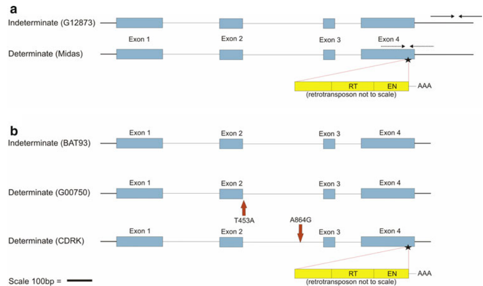
Fig. 1 Coding sequence (CDS) of determinate and indeterminate PvTFL1y haplotypes in common bean. a Haplotypes used in the cosegregation study. Solid line arrows used for genotyping a 6-bp indel in the F_2 population. Dashed line arrows used for genotyping the 4.1 kb retrotransposon. b Haplotypes used in the quantitative PCR and transformation studies. Arrows indicate single base pair substitutions. RT reverse transcriptase domain and EN endonuclease domain
